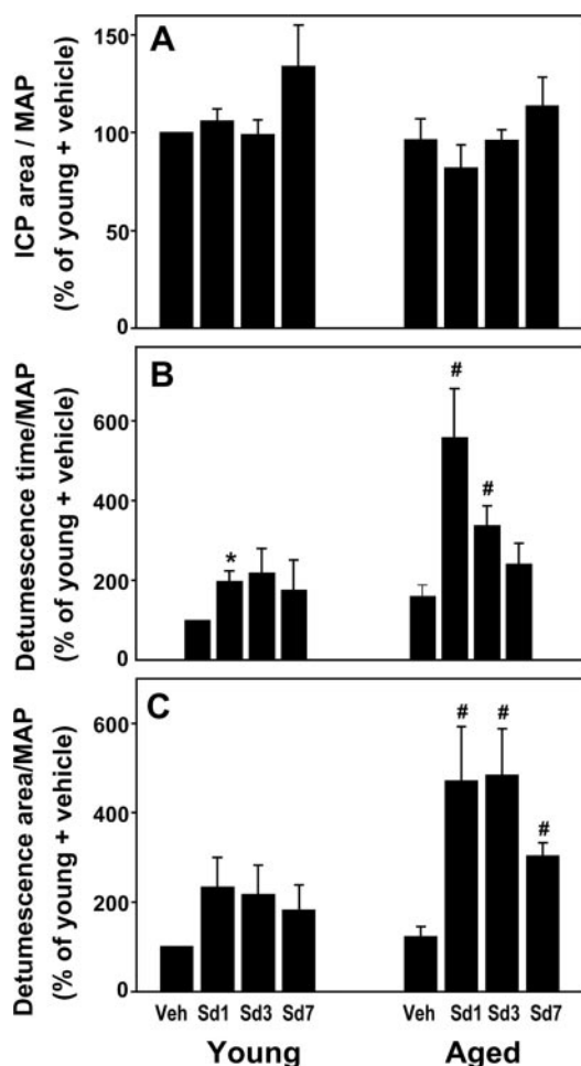
Fig. 1. Effect of long-term sildenafil treatment on erectile response. Young and aged rats were injected with sildenafil or saline subcutaneously every 8 h for 3 weeks. After a 1-, 3-, or 7-day washout period, a group of vehicle- and sildenafil-treated rats underwent electrical stimulation of the cavernous nerve to induce erection. Response parameters were expressed per MAP. ICP area is the area under the curve that corresponds to the duration of electrical stimulation; detumescence time is the period from the end of electrical stimulation to the point exhibiting 50% of maximal ICP; detumescence area is the area under the ICP curve during this interval. Values are normalized to young vehicle-treated; n = 5–6; *, p < 0.05 compared with young + vehicle; #, p < 0.05 compared with aged + vehicle. Veh, vehicle-treated; Sd1, Sd3, and Sd7 are responses on day 1, 3, and 7 washout after long-term sildenafil treatment.
